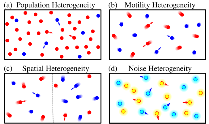
Figure 1. (color online) Schematic of the different heterogeneities applied on the TSVM. Particles of species A (B) are represented by red (blue) balls. (a) Population heterogeneity: N_A \neq N_B with v_A = v_B and \eta_A = \eta_B ; (b) Motility heterogeneity: v_A \neq v_B with N_A = N_B and \eta_A = \eta_B ; (c) Spatial heterogeneity: v_A > v_B in left region and v_A < v_B in right region, where the dotted line represents the inter-region interface, N_A = N_B and \eta_A = \eta_B ; (d) Noise heterogeneity: \eta_A \neq \eta_B with N_A = N_B and v_A = v_B , i.e. the red particles experience a higher noise amplitude (a “hotter” environment) compared to the blue particles (a “colder” environment).
