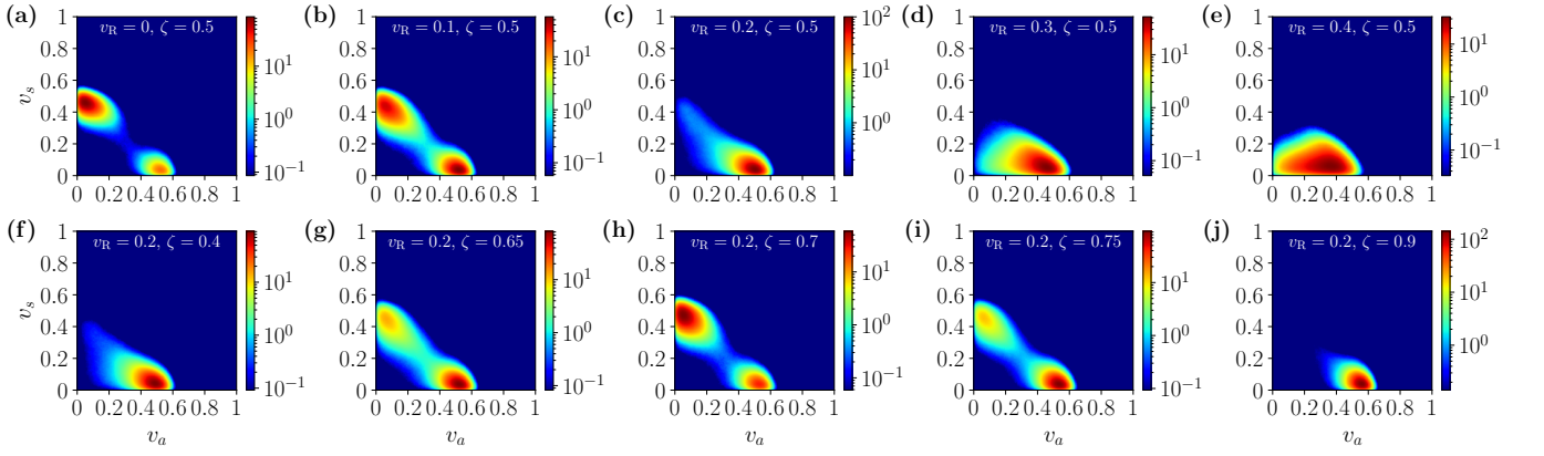
Figure 13. (color online) Probability distribution P(v_s, v_a) for spatial heterogeneity . (a–e) For constant \zeta = 0.5 and varying v_R . (f–j) For constant v_R = 0.2 and varying \zeta . Parameters: \rho = 0.5 , \eta = 0.24 , v_B = 0.5 , L_x = 256 , and L_y = 32 . Movies (Movie S3 and Movie S4) of the same can be found at Ref. [53].
