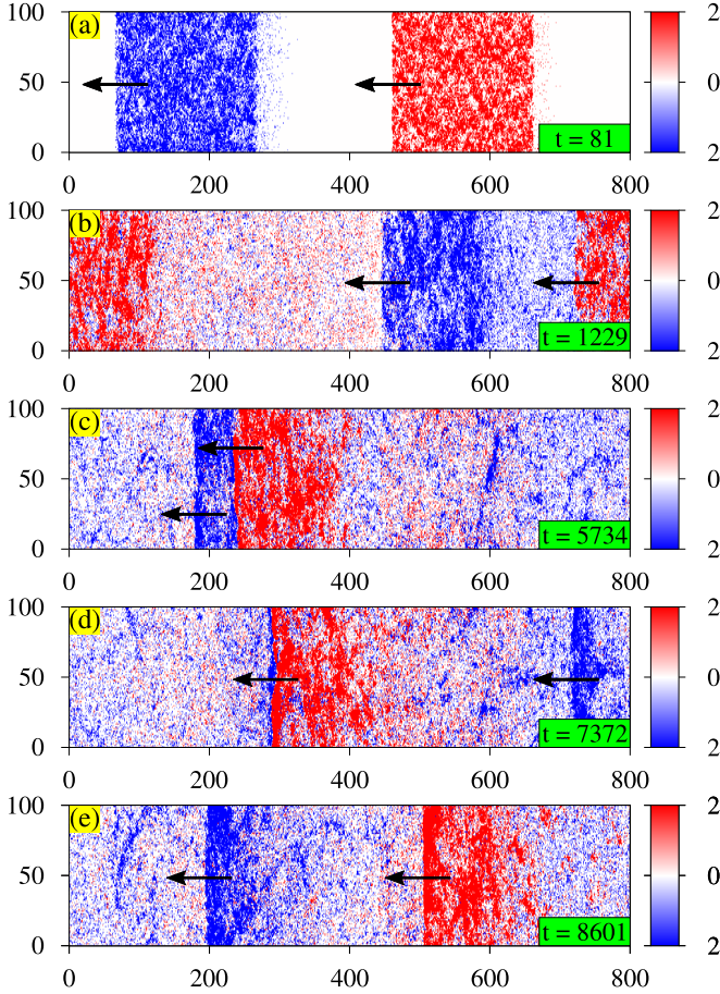
Figure 15. (color online) Time evolution of the TSVM under noise heterogeneity. (a) Initially, the bands of two species are in a PF state. (b–c) Over time, species A (red), having a higher group velocity, catches up to species B (blue), leading to a collision-mediated transition. (d–e) This interaction disrupts the flocking band of species B, causing fragmentation and subsequent reorganization into a new PF state. Parameters: \rho = 1 , \eta = 0.3 , v_0 = 0.5 , \Delta\eta = -0.2 , L_x = 800 , and L_y = 100 . A movie (movie4) of the same can be found at Ref. [52].
