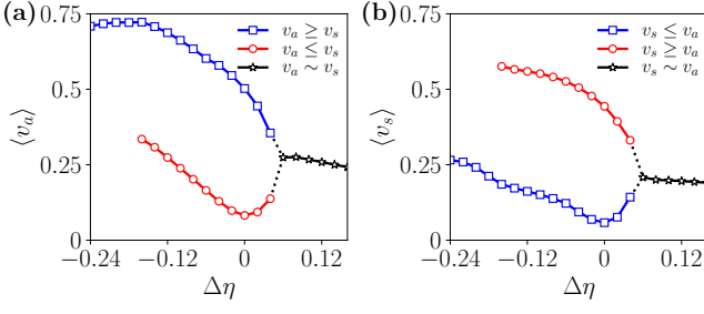
Figure 17. (color online) Order parameters for noise heterogeneity. \langle v_a \rangle and \langle v_s \rangle in the restricted APF (blue square), PF (red circle), and SSF (black star) ensembles for varying \Delta\eta . Parameters: \rho = 0.5 , \eta = 0.24 , v_0 = 0.5 , L_x = 256 , and L_y = 32 .
