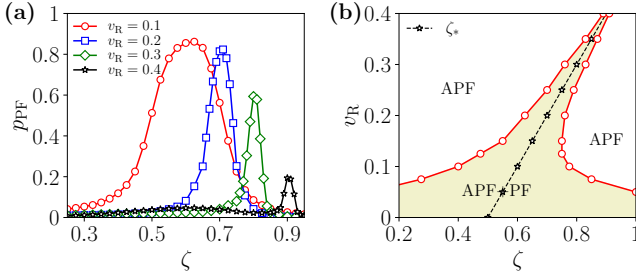
Figure 14. (color online) PF state probability and phase diagram for spatial heterogeneity . (a) p_{PF} versus \zeta for L_x = 256 and L_y = 32 . On increasing v_R , the peaks move towards higher \zeta and become thinner. (b) v_R - \zeta phase diagram. The shaded region denotes the APF+PF regime, while the black dotted line represents \zeta_* . Parameters: \rho = 0.5 , \eta = 0.24 , and v_B = 0.5 .
