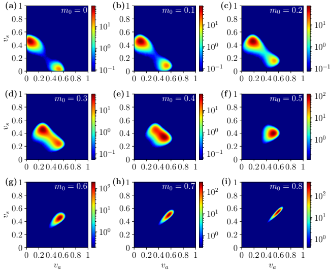
Figure 3. (color online) Probability distribution P(v_s, v_a) for varying population heterogeneity. (a) Representation of the homogeneous TSVM ( N_A = N_B ) exhibiting stochastic switching between the PF and APF states. (b–i) The two peaks progressively converge as m_0 increases, signifying a collapse into a single state. Parameters: \rho = 0.5 , \eta = 0.24 , v_0 = 0.5 , L_x = 256 , and L_y = 32 . A movie (Movie S1) of the same can be found at Ref. [53].
