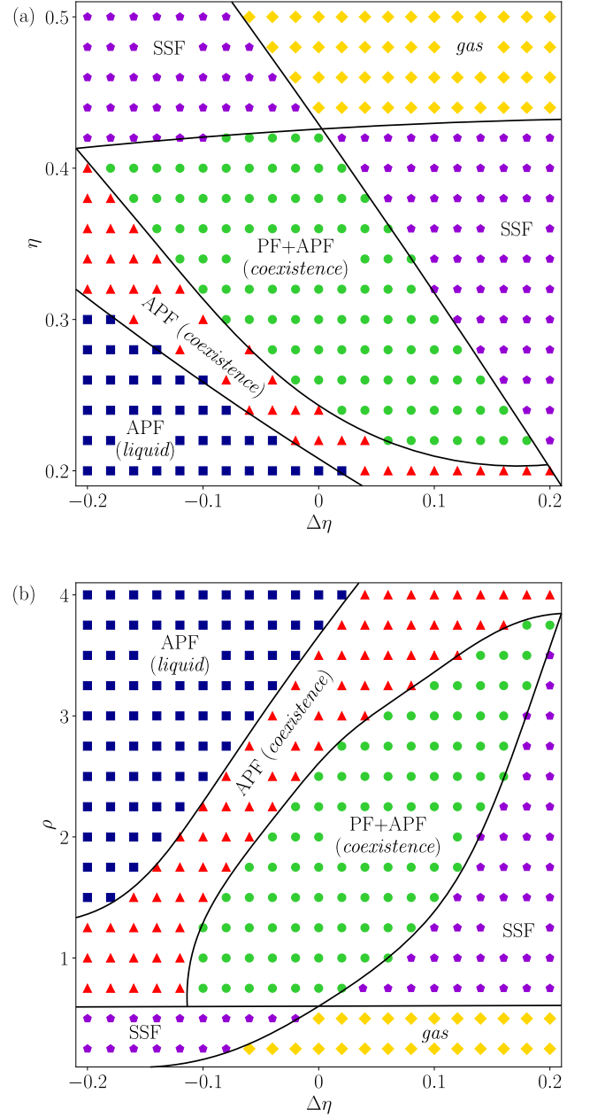
Figure 18. (color online) Phase diagrams for noise heterogeneity. (a) \eta - \Delta\eta phase diagram for fixed \rho = 1.5 ; (b) \rho - \Delta\eta phase diagram for fixed \eta = 0.3 . For both cases, the velocity moduli is v_0 = 0.5 . The boundary lines act as a guide to the eyes.
