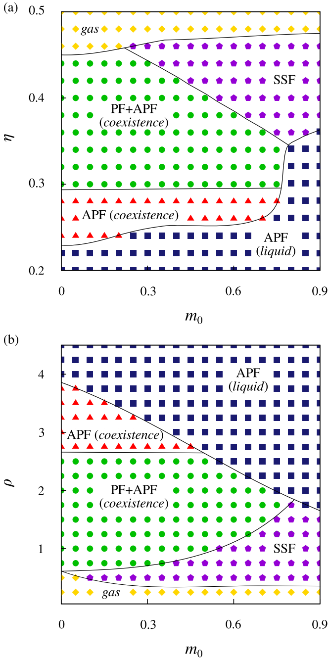
Figure 6. (color online) Phase diagrams for population heterogeneity. (a) \eta - m_0 phase diagram for \rho = 2 ; (b) \rho - m_0 phase diagram for \eta = 0.3 . For both cases, the velocity moduli is fixed ( v_0 = 0.5 ). Alongside the homogeneous TSVM phases, a single-species flocking state emerges. The boundary lines are included as visual guides.
