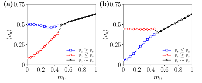
Figure 4. (color online) Order parameters for population heterogeneity. \langle v_a \rangle and \langle v_s \rangle are shown in the restricted APF (blue squares), PF (red circles), and SSF (black stars) ensembles for varying m_0 . (a) \langle v_a \rangle remains relatively constant in the APF ensemble but increases monotonically in the PF ensemble. (b) \langle v_s \rangle increases monotonically in the APF ensemble while remaining relatively constant in the PF ensemble. Parameters: \rho = 0.5 , \eta = 0.24 , v_0 = 0.5 , L_x = 256 , and L_y = 32 .
