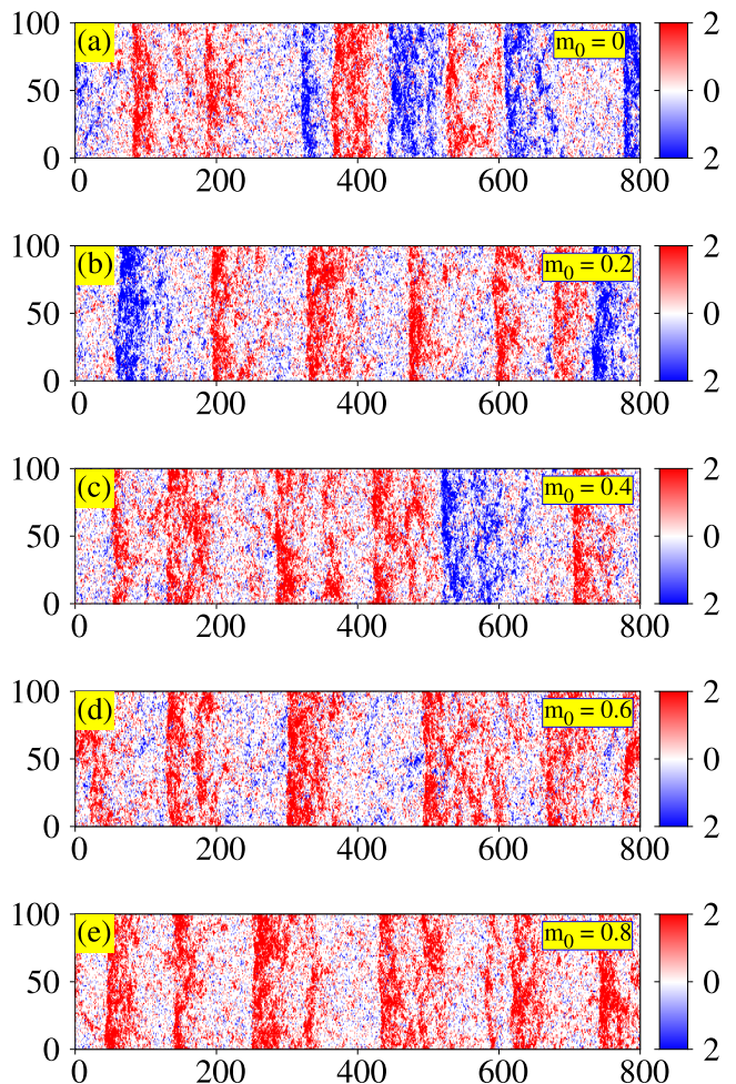
Figure 2. (color online) Steady-state snapshots for varying population heterogeneity. Particles of species A (B) are represented with red (blue) dots, and a local particle density is color-coded according to the color bar. (a) The homogeneous TSVM features an equal number of bands for A and B species. (b–c) The band number of species B decreases with increasing m_0 . (d–e) B-particles can not form bands due to scarcity in numbers. Parameters: \rho = 1 , \eta = 0.3 , v_0 = 0.5 , L_x = 800 , and L_y = 100 . A movie (movie1) of the same can be found at Ref. [52].
