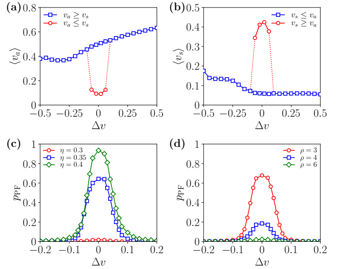
Figure 9. (color online) Order parameters and PF state probability for motility heterogeneity. (a) \langle v_a \rangle and (b) \langle v_s \rangle in the restricted APF (blue square) and PF (red circle) ensembles versus \Delta v for \rho = 0.5 and \eta = 0.24 . (c-d) Probability of the PF state ( p_{\text{PF}} ) vs \Delta v for (c) varying noise strength \eta [ = 0.30 (circle), 0.35 (square) and 0.40 (diamond)] keeping \rho = 2 fixed and (d) varying particle density \rho [ = 3 (circle), 4 (square) and 6 (diamond)] keeping \eta = 0.4 fixed. Parameters: v_0 = 0.5 , L_x = 256 , and L_y = 32 .
