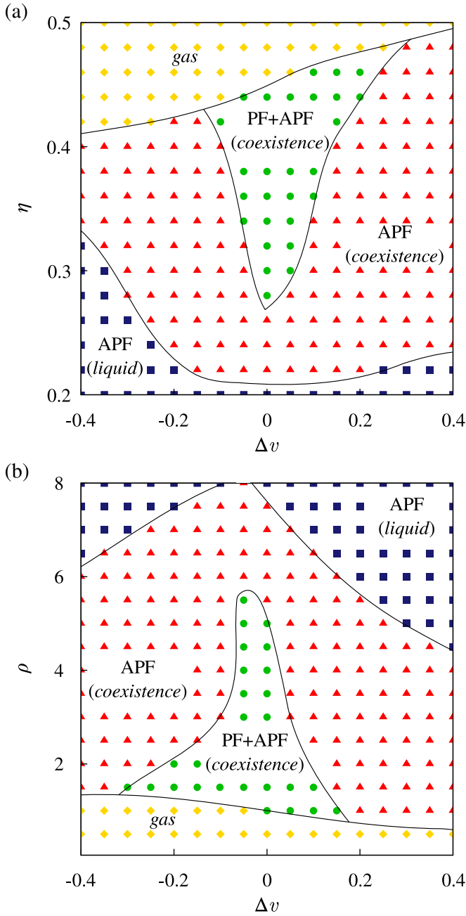
Figure 10. (color online) Phase diagrams for motility heterogeneity. (a) \eta - \Delta v phase diagram for fixed \rho = 1.5 ; (b) \rho - \Delta v phase diagram for fixed \eta = 0.4 . For both cases, the velocity moduli of B species is fixed ( v_B = 0.5 ). The boundary lines act as a guide to the eyes.
