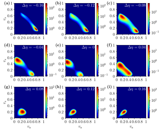
Figure 16. (color online) Probability distribution P(v_s, v_a) for varying noise heterogeneity. (a–b) shows PF-APF stochastic switching with strong APF behavior and strong ordering. (c–f) denotes this switching with more prominence of PF behavior as \Delta\eta increases. (g–i) demonstrates the dissolution of the dual flocking states as the system shows a SSF state at high \Delta\eta . Parameters: \rho = 0.5 , \eta = 0.24 , v_0 = 0.5 , L_x = 256 , and L_y = 32 . A movie (Movie S5) of the same can be found at Ref. [53].
