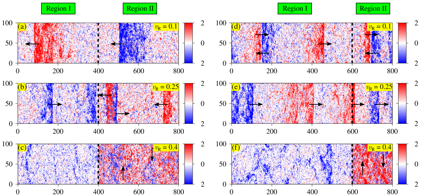
Figure 12. (color online) Steady-state snapshots for spatial heterogeneity. A (B) particles are represented by red (blue) dots, with local particle density color-coded according to the color bar. Black arrows indicate the direction of flock propagation. The dashed vertical line separates the v_A > v_B region on the left from the v_A < v_B region on the right. (a–c) Equal region sizes ( \zeta = 0.5 ). (d–f) Unequal region sizes ( \zeta = 0.75 ). Parameters: \rho = 1 , \eta = 0.3 , v_B = 0.5 , L_x = 800 , and L_y = 100 . A movie (movi3) of the same can be found at Ref. [52].
