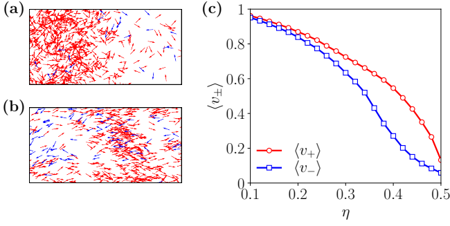
Figure 5. (color online) Single species and both species flocking at large population heterogeneity. Snapshots of (a) SSF ( \eta = 0.45 ) and (b) flocking of both species in an APF state ( \eta = 0.2 ) are shown for a 20 \times 10 section of a 800 \times 100 simulation box. Red and blue arrows represent the orientation of A and B particles, respectively. (c) The time- and ensemble-averaged order parameters \langle v_{\pm} \rangle as a function of \eta ; L_x = 256 , L_y = 32 . Parameters: \rho = 2 , v_0 = 0.5 , and m_0 = 0.9 .
