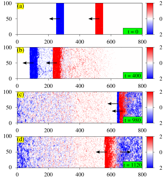
Figure 7. (color online) Time-evolution with motility heterogeneity. The flocking direction is indicated by black arrows. (a) Particles of species A (red dots) and species B (blue dots) are shown, with local particle density color-coded according to the color bar. (b–c) The faster-moving A-band catches the B-band and collides. (d) Species B reverses direction and forms an APF state. Parameters: \rho = 1 , \eta = 0.3 , v_0 = 0.5 , \Delta v = 0.3 , L_x = 800 , and L_y = 100 . A movie (movie2) of the same can be found at Ref. [52].
