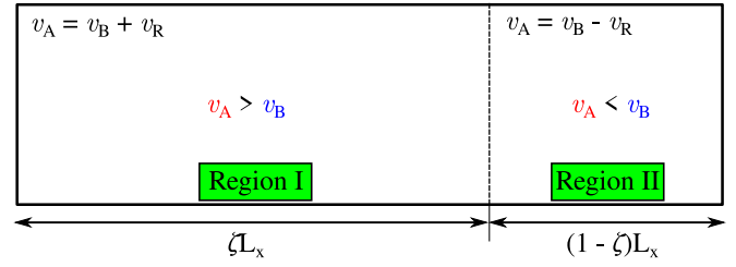
Figure 11. (color online) Schematic representation of the activity landscape. v_B is constant throughout the geometry. \zeta is the fraction of space where v_A > v_B . This arrangement ensures that A-particles change their velocity twice: once at the interface boundary (vertical dotted line) and again due to the periodic boundary condition.
